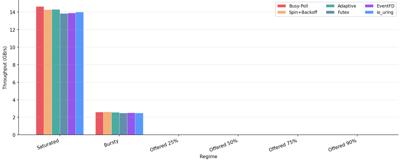
Fig. 5. Throughput by Variant and Arrival Regime. Throughput collapses from \approx 14 GiB/s under saturated load to near-zero under offered-load sweeps as the ring empties between arrivals, regardless of wakeup mechanism.
