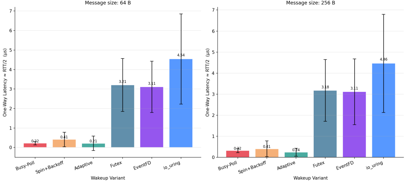
Fig. 3. Ping-Pong Latency Across All Six SHM Wakeup Variants. Spinning variants achieve sub-microsecond latency at small sizes; kernel-sleeping variants converge to 3\text{--}5 \mu\text{s} . All six converge near 150\text{--}155 \mu\text{s} at 1 MiB, confirming memory bandwidth as the common bottleneck.
